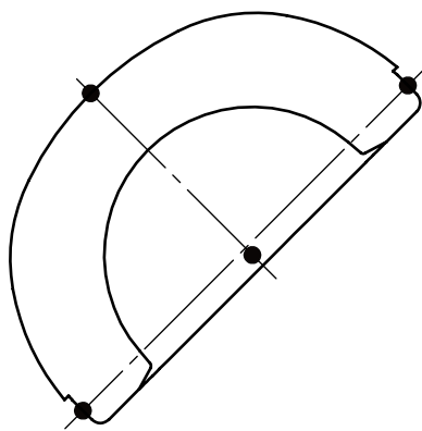
Size 56 (Head Ø36)
